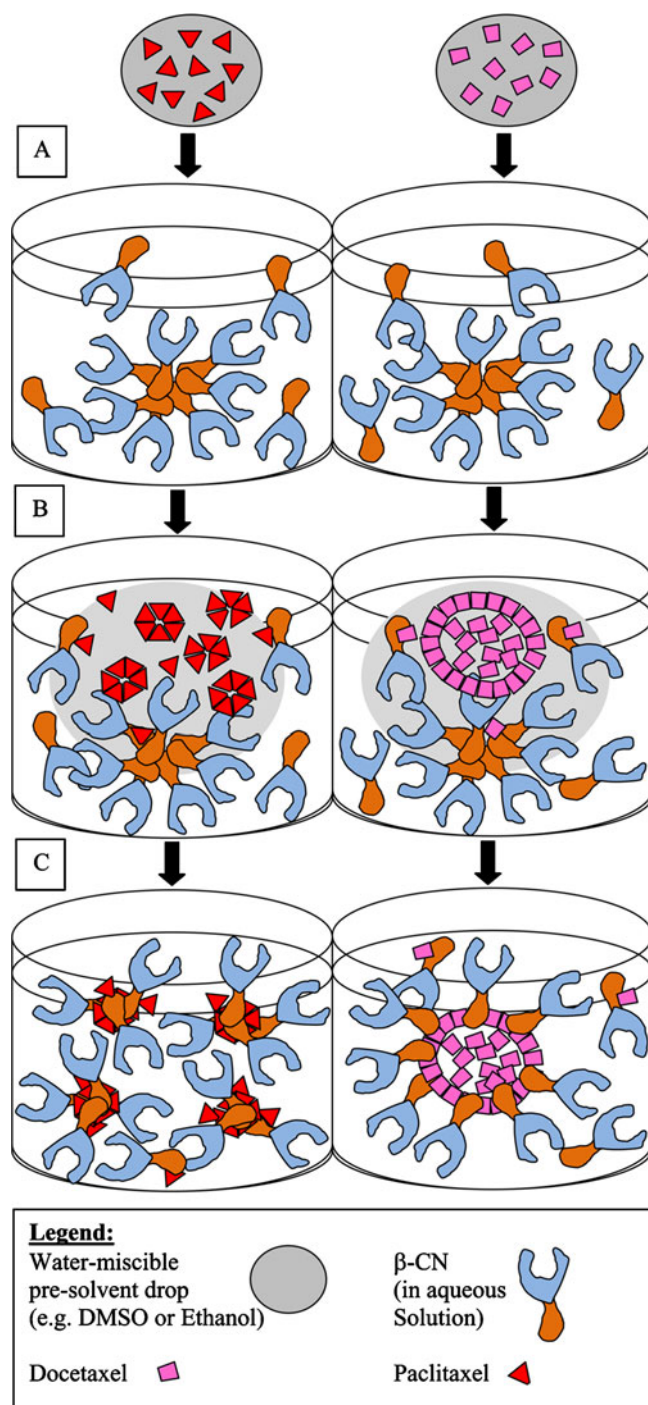
Fig. 11 A schematic diagram modeling the proposed sequence of events occurring during addition of the uncharged hydrophobic drugs, dissolved in a water-miscible solvent (DMSO or ethanol) into aqueous \beta -CN solution: A. The two drugs are well dissolved in the solvent. B. Upon addition to the aqueous solution, the solvent starts dissipating, and the drugs consequently self-assemble by the hydrophobic effect. Apparently, the geometry and better amphiphilicity of paclitaxel causes it to form smaller “primary micellar aggregates” compared to docetaxel. C. \beta -CN then “wraps” these primary aggregates, and stabilizes them, preventing their further aggregation. The smaller primary particles formed by paclitaxel result in smaller final nanocapsules.
