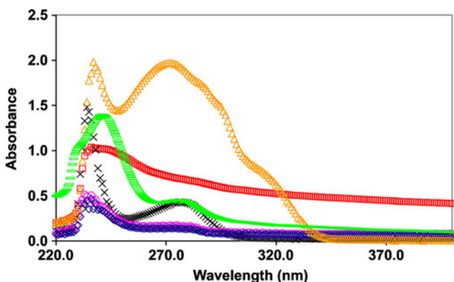
Fig. 2 Spectra of absorbance of 167 \mu M pure paclitaxel ( \square ), docetaxel ( \circ ), vinblastine ( \Delta ), irinotecan ( \diamond ), 42 \mu M mitoxantrone (—) and 1 mg/ml (42 \mu M) pure \beta -CN ( \times ).
