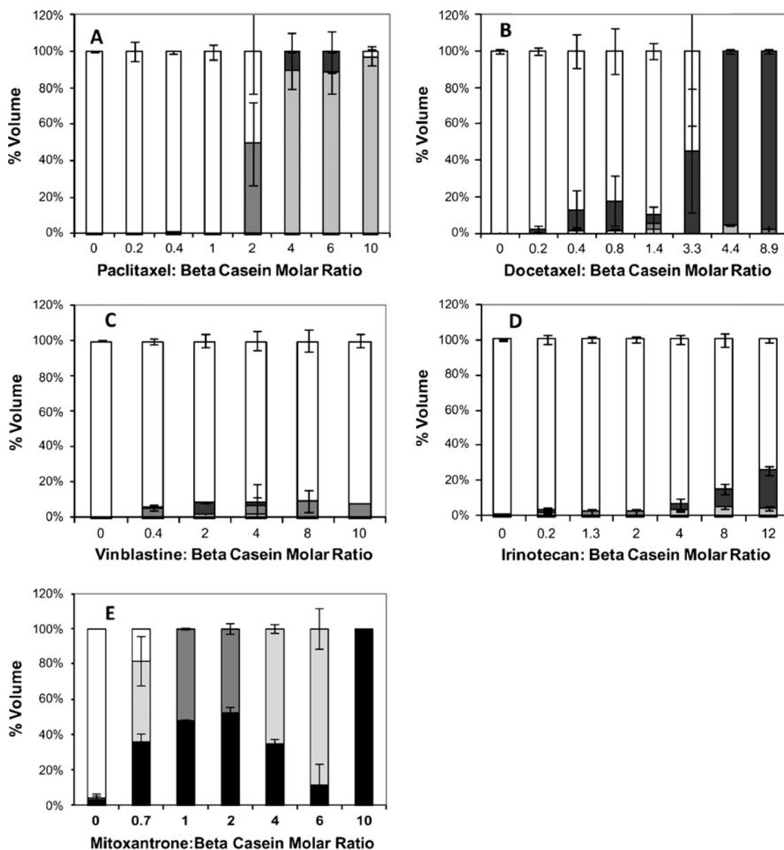
Fig. 9 Drug- \beta -CN particle size distribution. Volume percentage as a function of drug: \beta -CN molar ratio, in 1 mg/ml \beta -CN. (□) 0–100 nm, (▨) 100–200 nm, (▩) 200–300 nm, (■) 300 nm and up. (A) paclitaxel- \beta -CN nano particles, (B) docetaxel- \beta -CN nano particles, (C) vinblastine- \beta -CN nano particles, (D) irinotecan- \beta -CN nano particles and (E) mitoxantrone- \beta -CN nano particles (8).
