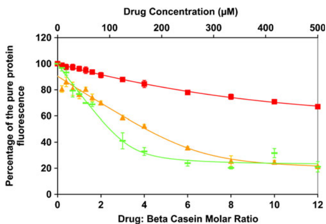
Fig. 5 Percentage of the initial Trp 143 emission as a function of drug concentration ( top axis ) and drug: β-CN molar ratio ( bottom axis ) of paclitaxel (■), vinblastine (▲), and mitoxantrone (●) in a 1 mg/ml β-CN solution. (Excitation: 287 nm and emission: 332 nm.) Line represents the model fit.
